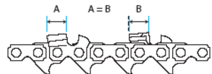
Figure 42: Keep cutters equal
