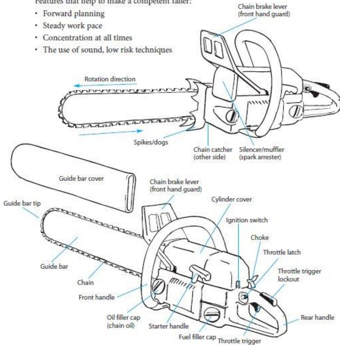
Figure 1: Components of a chainsaw
