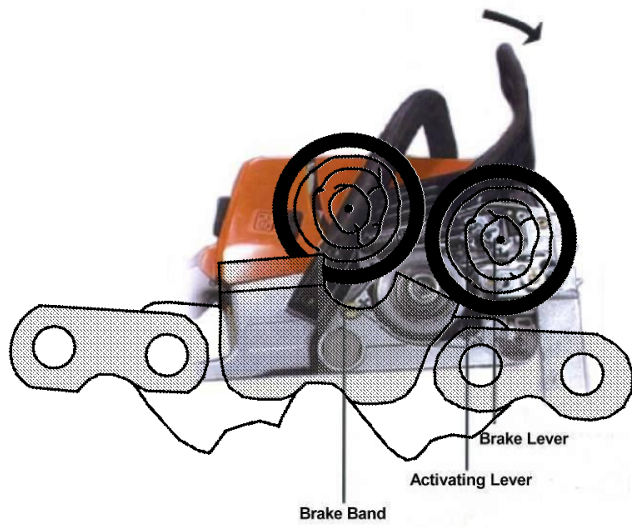
Figure 2: Chain brake mechanism
