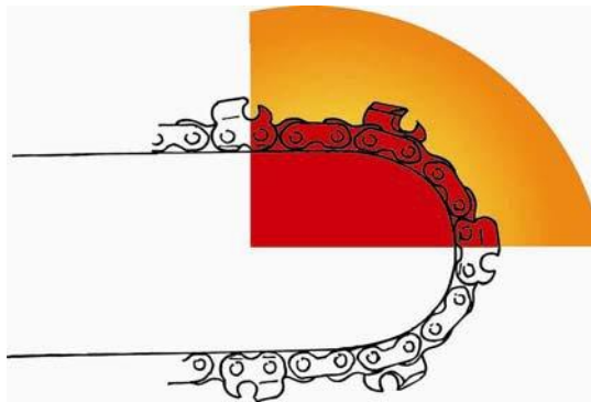
Figure 56: Kickback reaction zone
