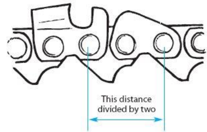
Figure 24: Measuring the pitch
