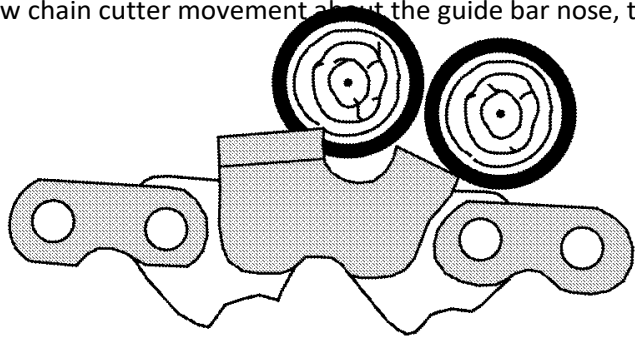
Figure 3: Modern low kickback tendency chain
