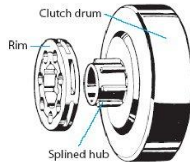
Figure 21: Fitting a rim drive sprocket
