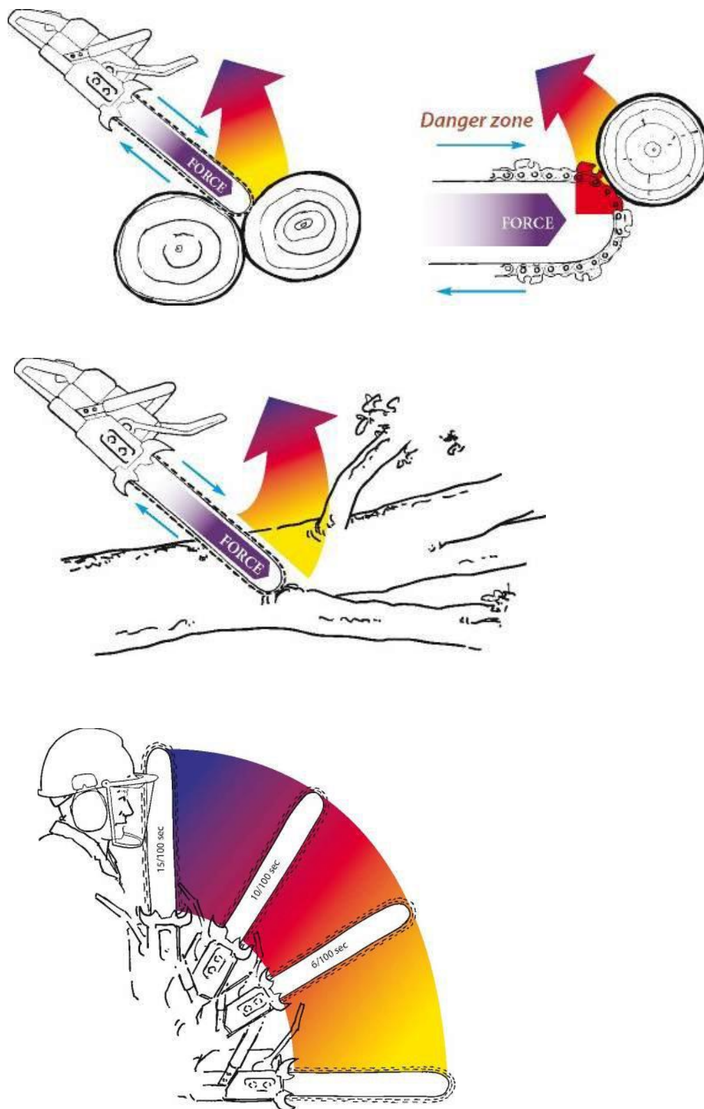
Figure 57: Common kickback situations
