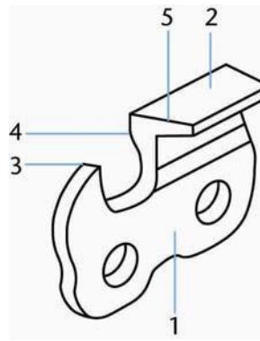
Figure 33: Parts of a cutter
