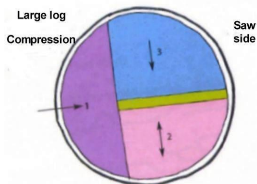
Figure 76: Cross cutting of log with side bind
