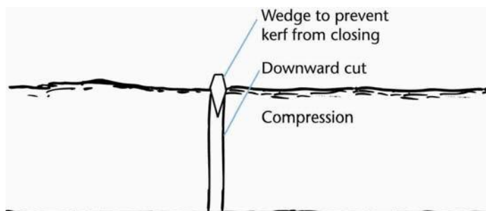
Figure 75: Cross cut large log lying on ground
