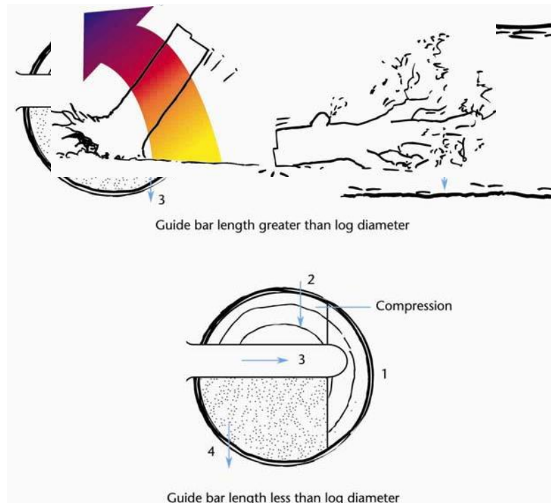
Figure 77: Plunge cutting technique - Method of cross cutting for log quality
