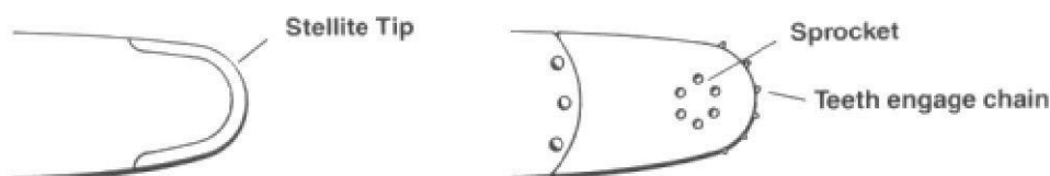
Figure 26: Solid nose and sprocket nose guide bars
