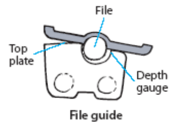
Figure 41: Positioning the guide
