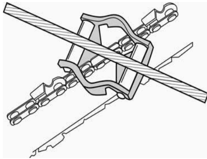
Figure 39: Roller file guide
