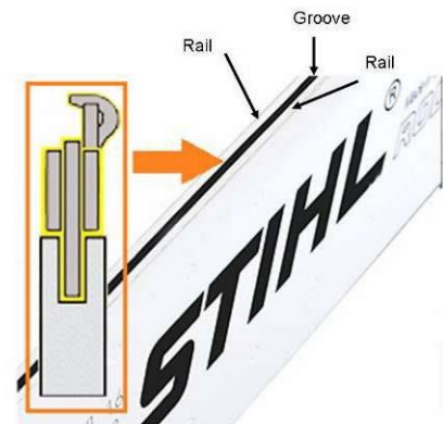
Figure 25: Guide bar
