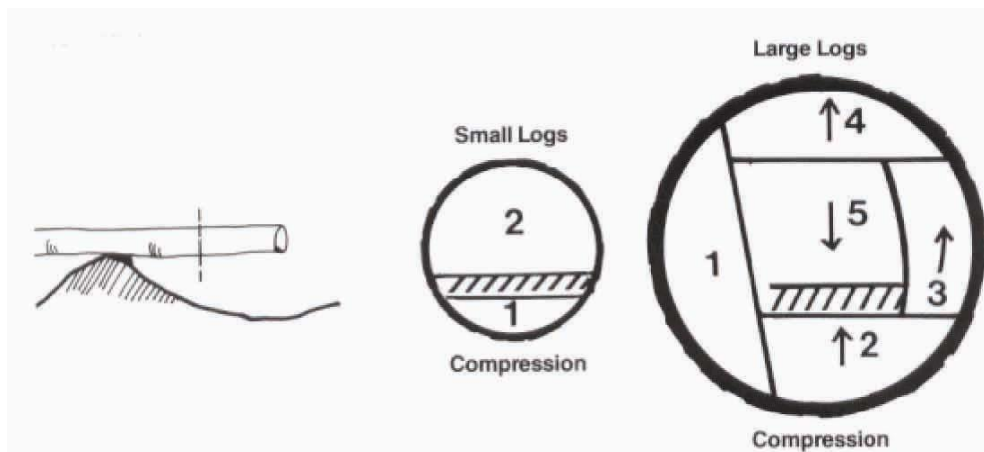
Figure 73: Hanging trunk section supported at one end only
