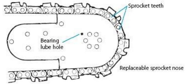
Figure 27: Replaceable sprocket nose guide bar
