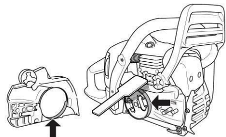
Figure 17: Cleaning the chain brake
