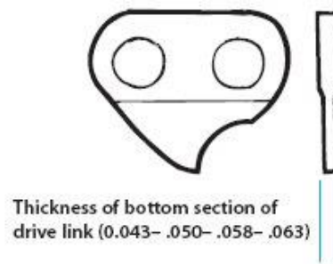
Figure 36: Drive link gauge
