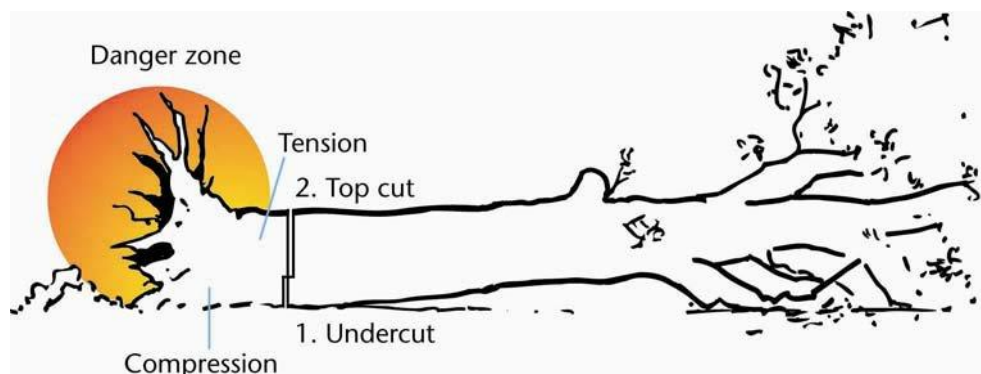
Figure 80: Place stagger cut as close as possible to root mass
