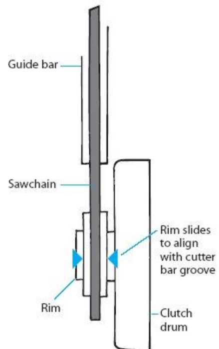
Figure 22: Alignment of drive sprocket
