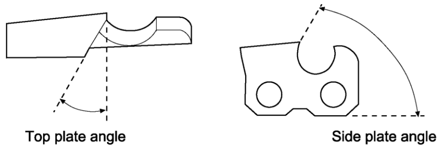
Figure 43: Filing angles
