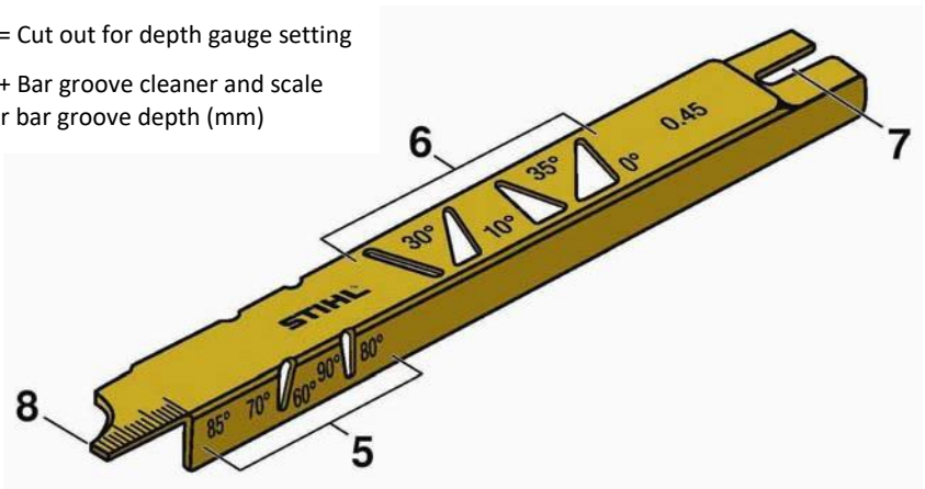
Figure 40: Conventional file guide
