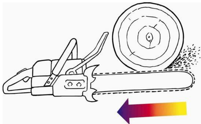
Figure 54: Chainsaw push-back reaction
