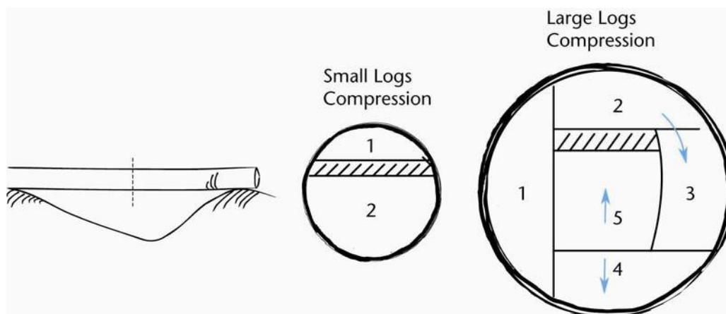
Figure 71: Cross cut trunk section supported at both ends
