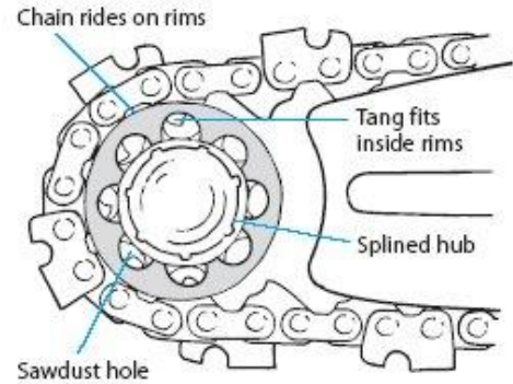
Figure 20: Rim (floating) drive sprocket
