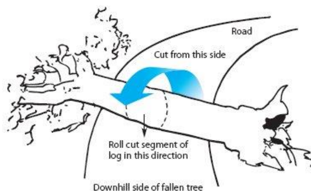
Figure 74: Crosscutting a small log
