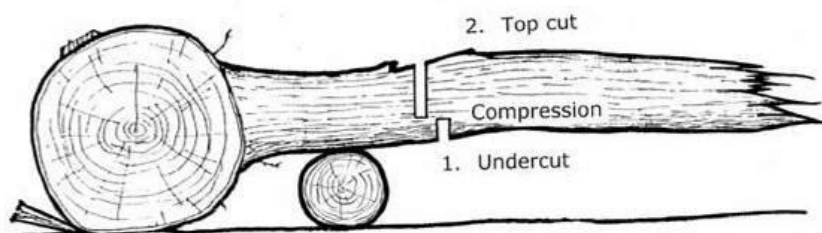
Figure 65: Method of removing a heavy horizontal limb supported at one end only
